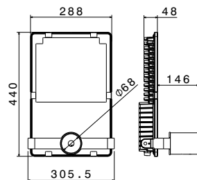
Integrated pole-top mounting
